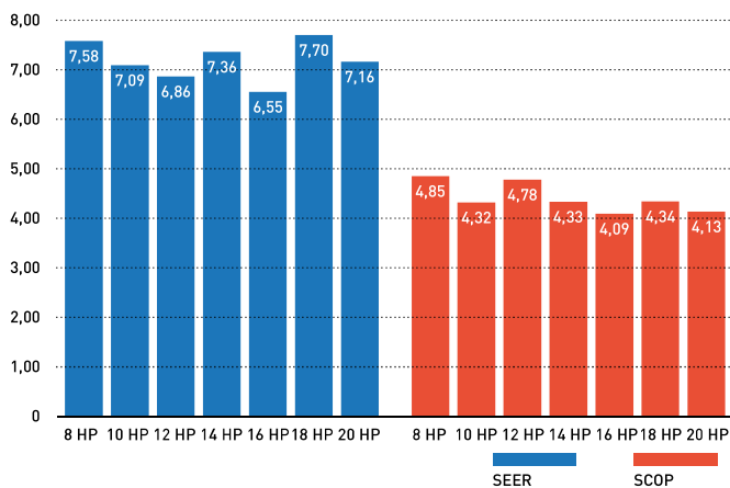
SEER / SCOP
